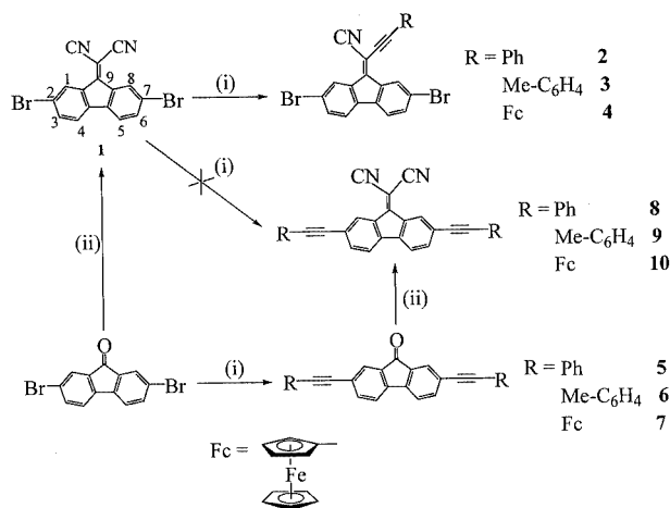
Scheme 1. (i) \text{RC}\equiv\text{CH} , \text{Pd}(\text{OAc})_2 , \text{PPh}_3 , \text{CuI} , i\text{Pr}_2\text{NH} ; (ii) \text{CH}_2(\text{CN})_2 , DMSO, 110 °C
